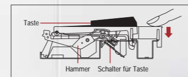
Progressive Hammer-Action-Tastatur
